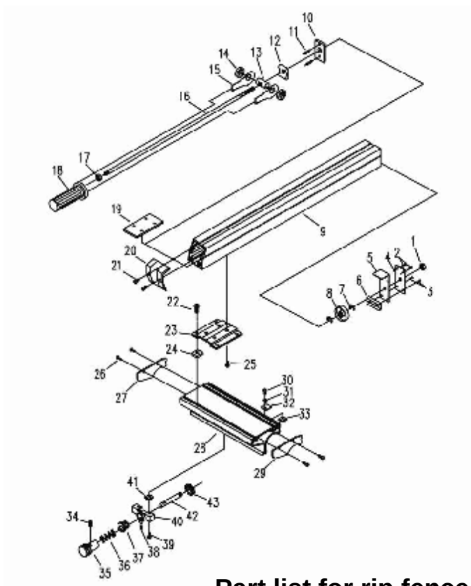
Part list for rip fence
